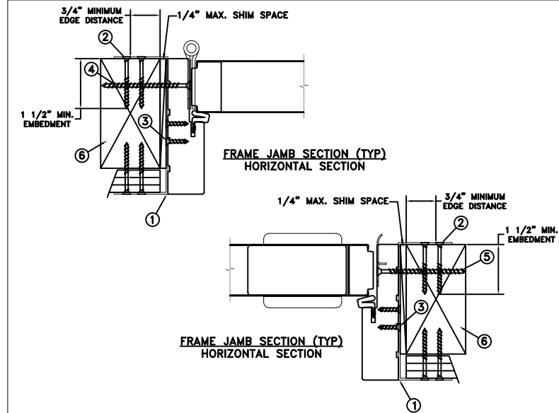
MASONRY STRAP INSTALLATION
