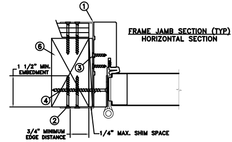
FRAME JAMB SECTION (TYP) HORIZONTAL SECTION
